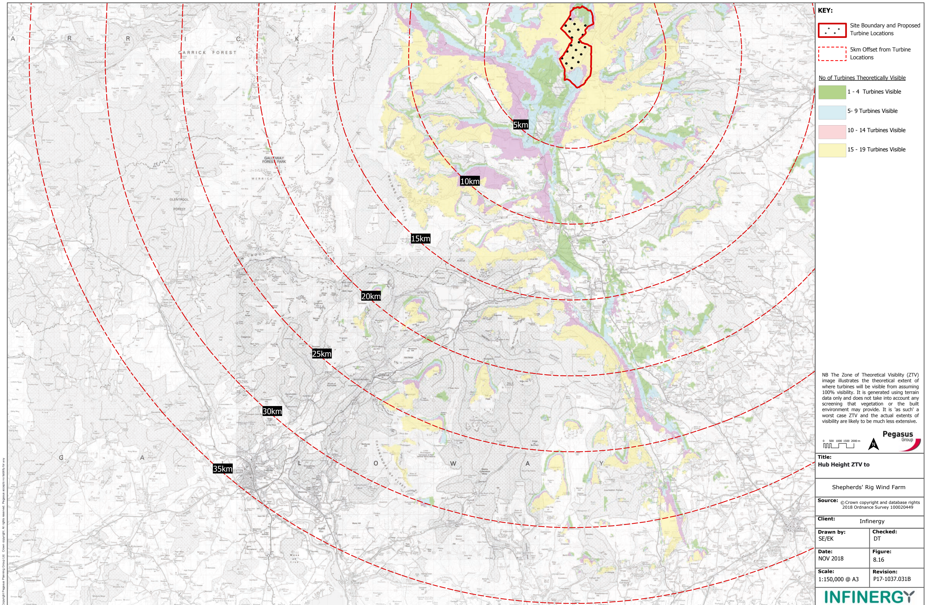
Figure 8.16 Hub Height ZTV to 35 km (SW Quadrant)
